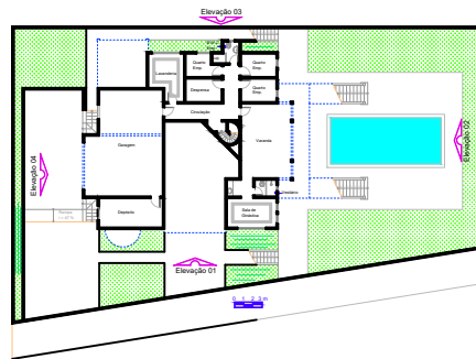
Subsolo A = 200,83 m 2
